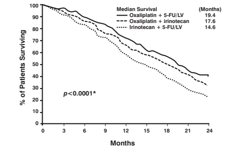
Figure 4 – Kaplan-Meier Overall Survival by treatment arm
